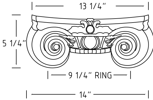
8" COLUMN
